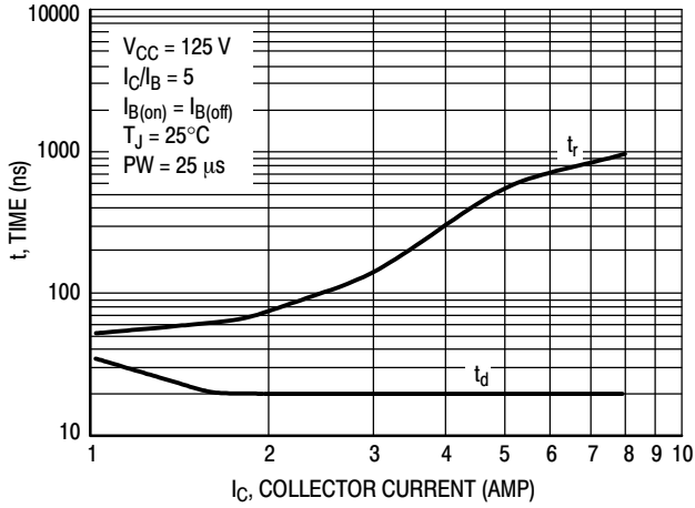
Figure 10. Turn-On Time (Resistive Load)
