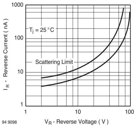
Figure 3. Reverse Current vs. Reverse Voltage
